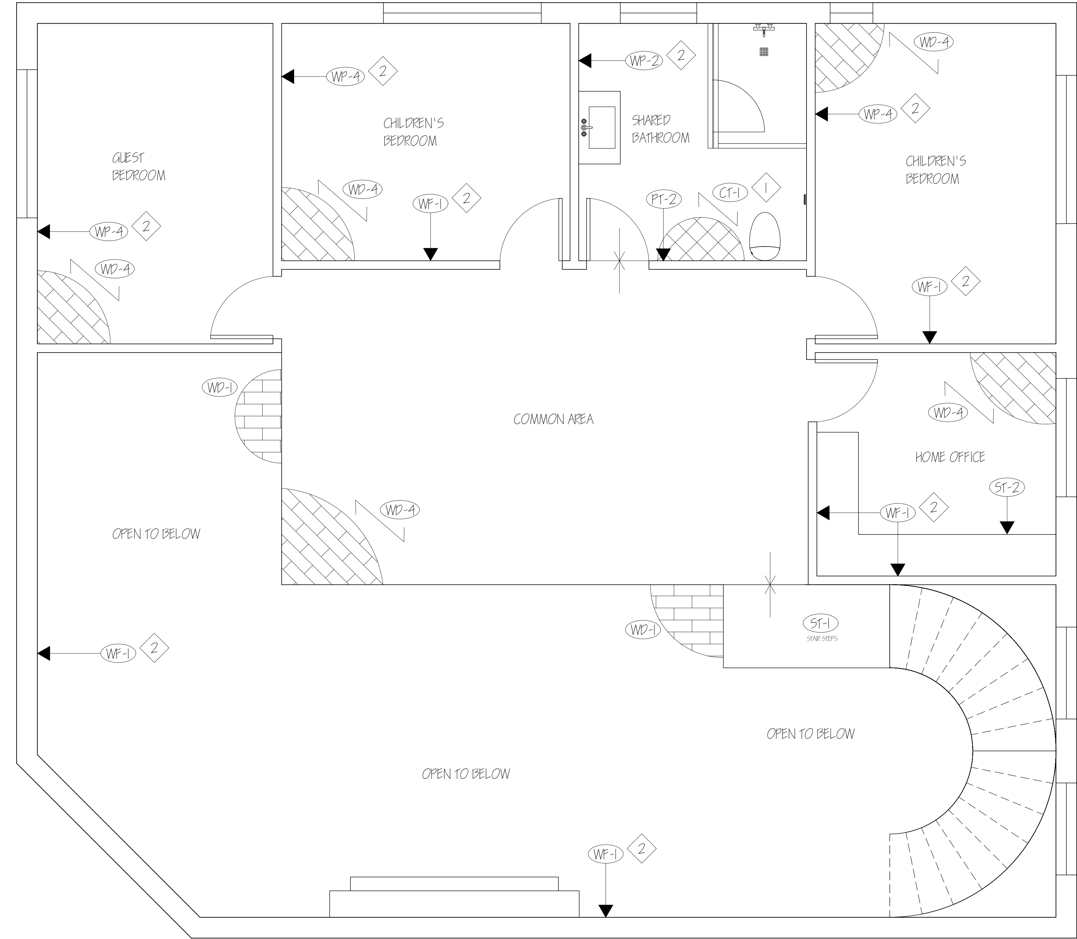
1 2ND FLOOR MATERIAL FINISH PLAN SCALE: \frac{1}{4}" = 1'-0"
