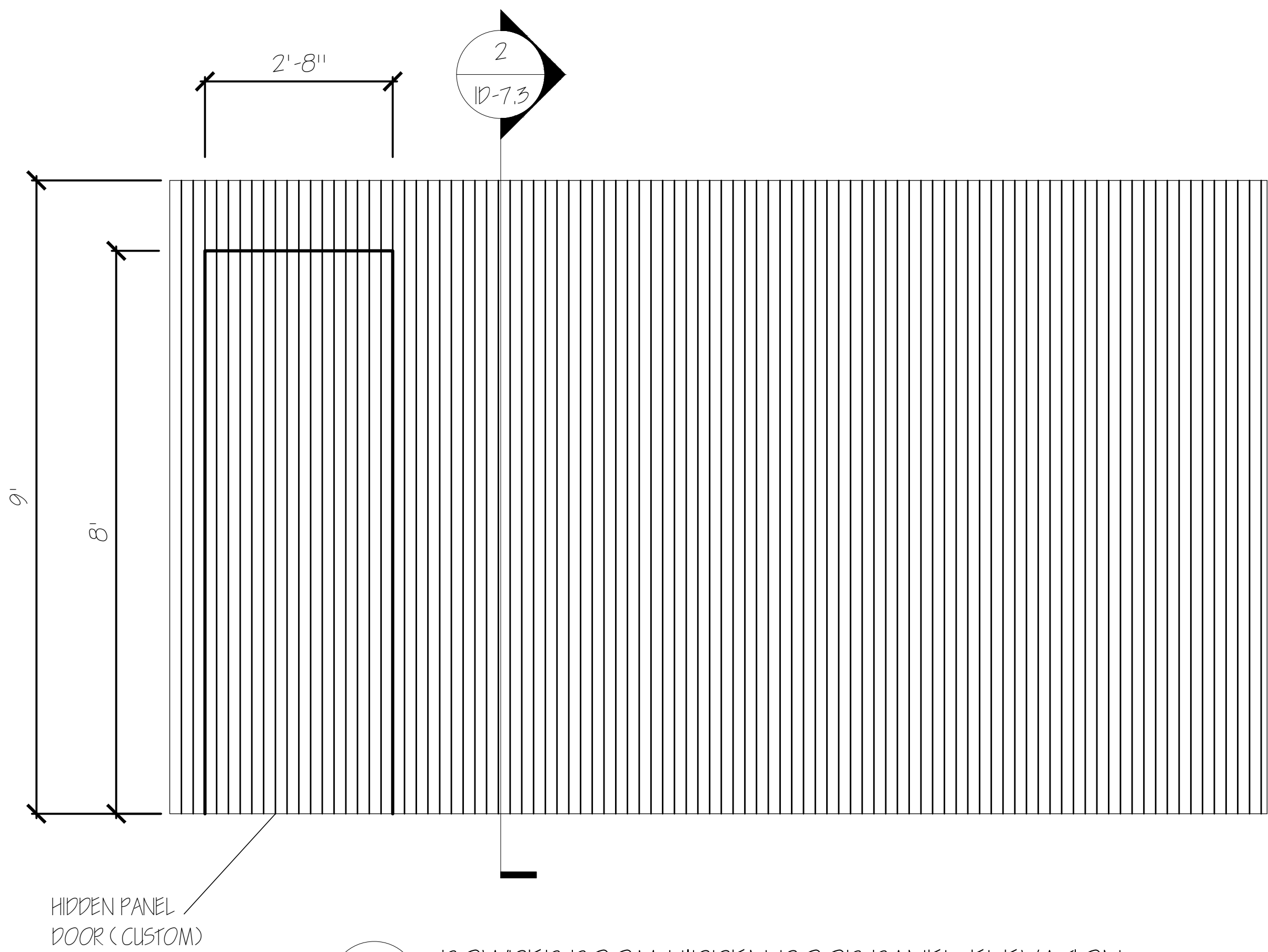
1 POWDER ROOM HIDDEN DOOR PANEL ELEVATION SCALE: \frac{1}{2} " = 1'-0"
