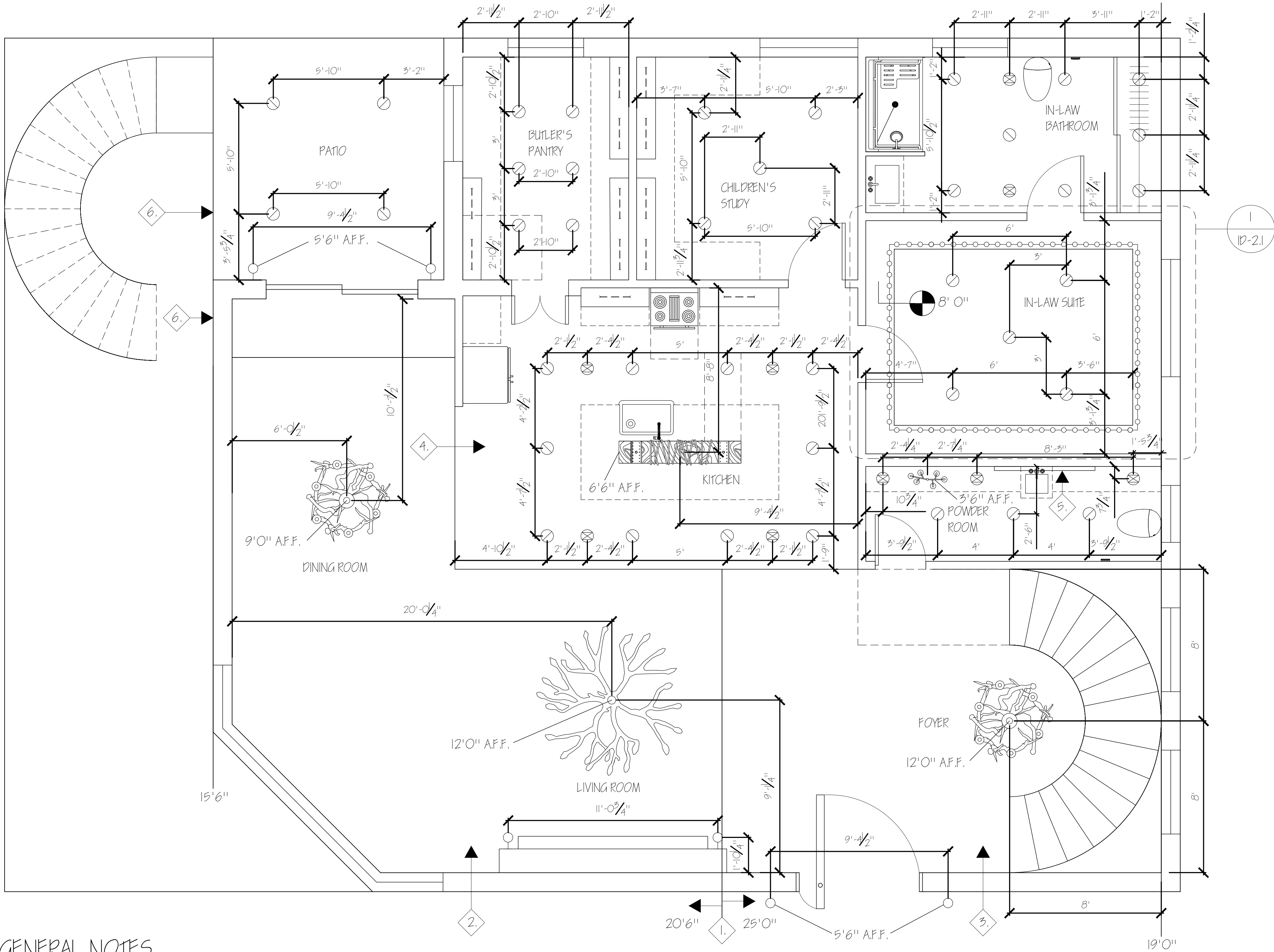
1 1ST FLOOR FINAL RCP SCALE: 1/4" = 1'-0"
