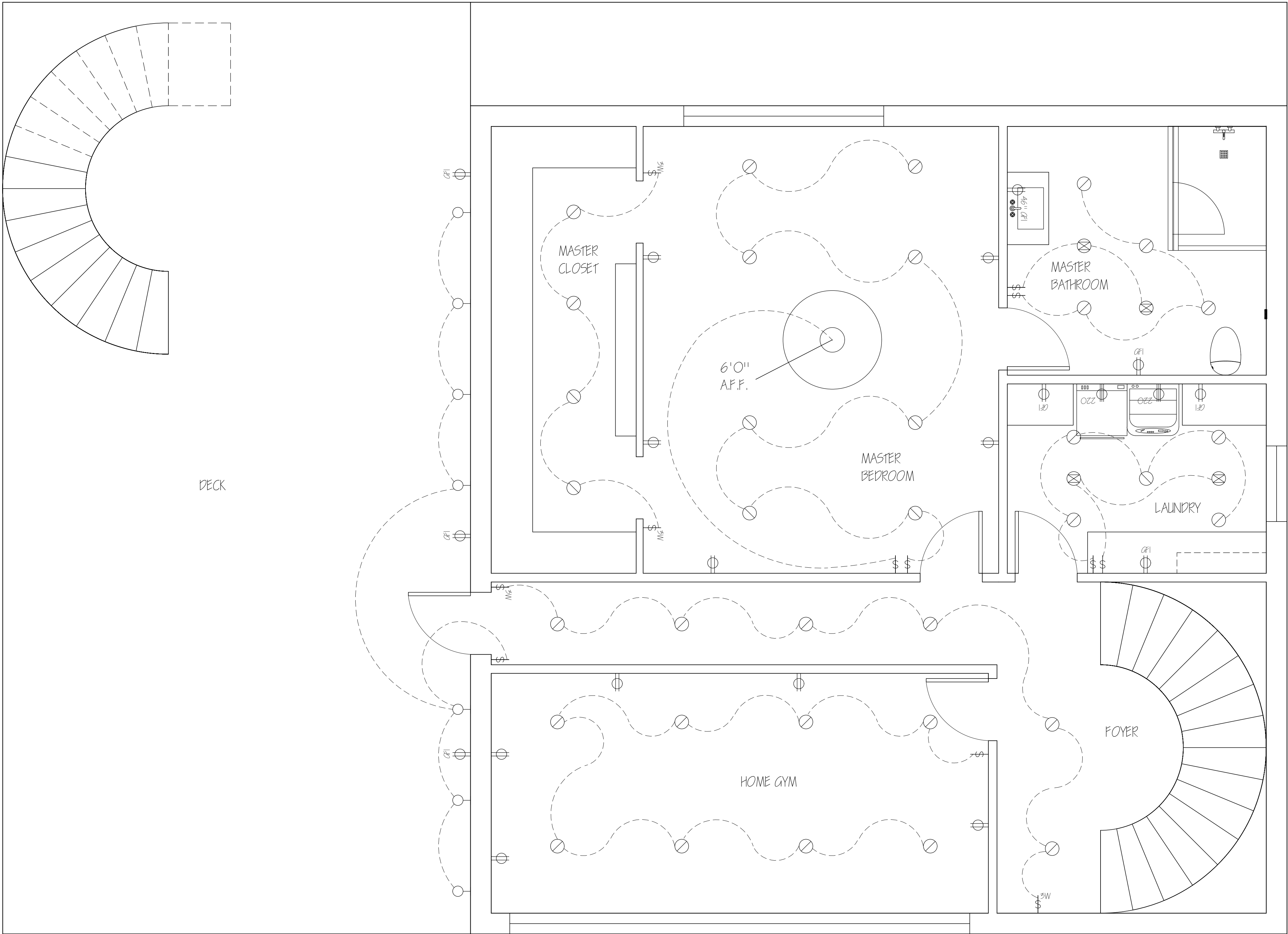
1 BASEMENT ELECTRICAL PLAN SCALE: \frac{1}{4}" = 1'-0"
