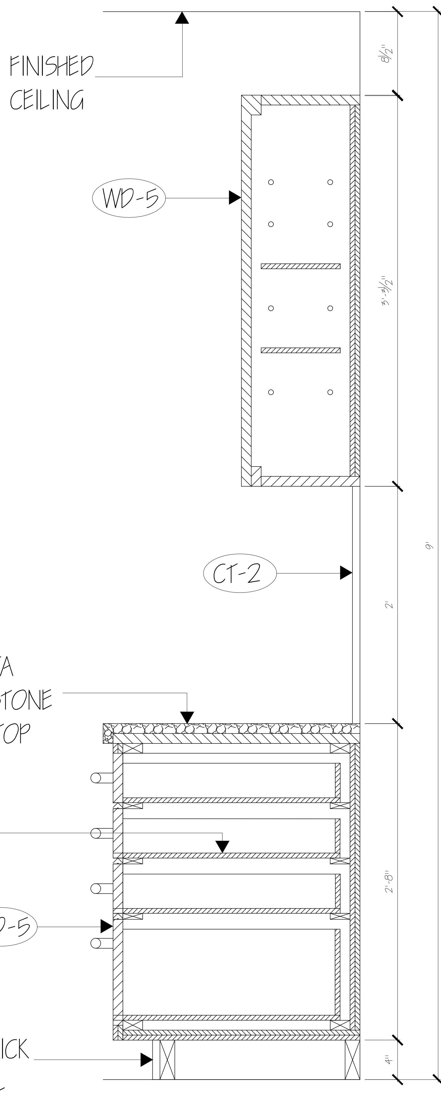
1 KITCHEN CABINET SECTION SCALE: \frac{1}{2}" = 1'-0"
