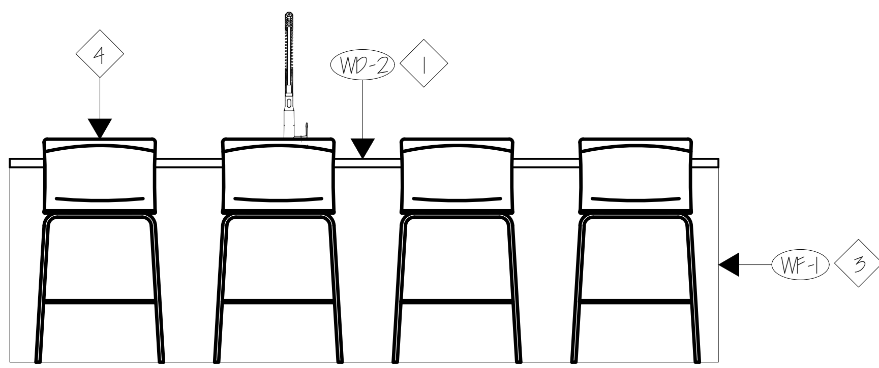
2 KITCHEN ISLAND REAR VIEW ELEVATION SCALE: \frac{1}{2} " = 1'-0"
