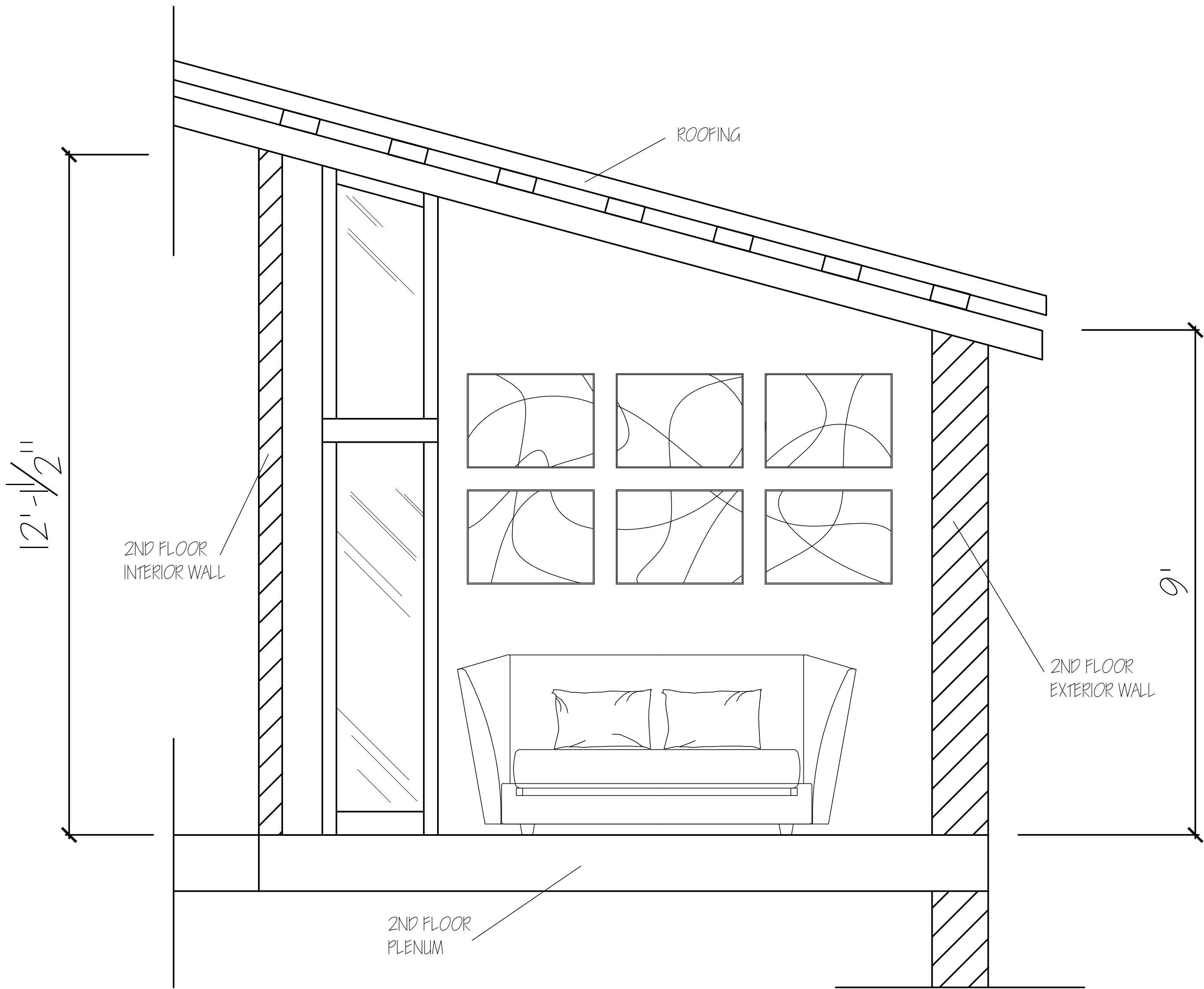
1 CHILDREN'S BEDROOM SECTION C-C CUT SCALE: 1/2" = 1'-0"
