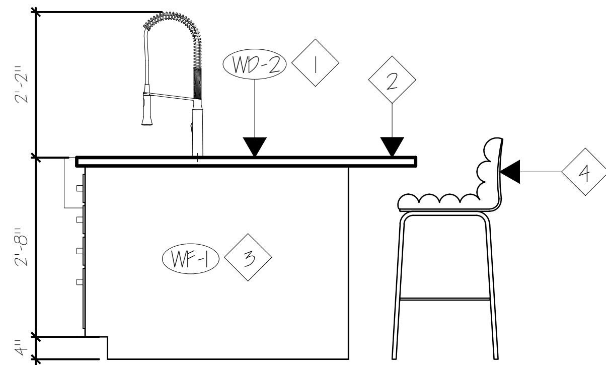
1 KITCHEN ISLAND RIGHT VIEW ELEVATION SCALE: \frac{1}{2} " = 1'-0"
