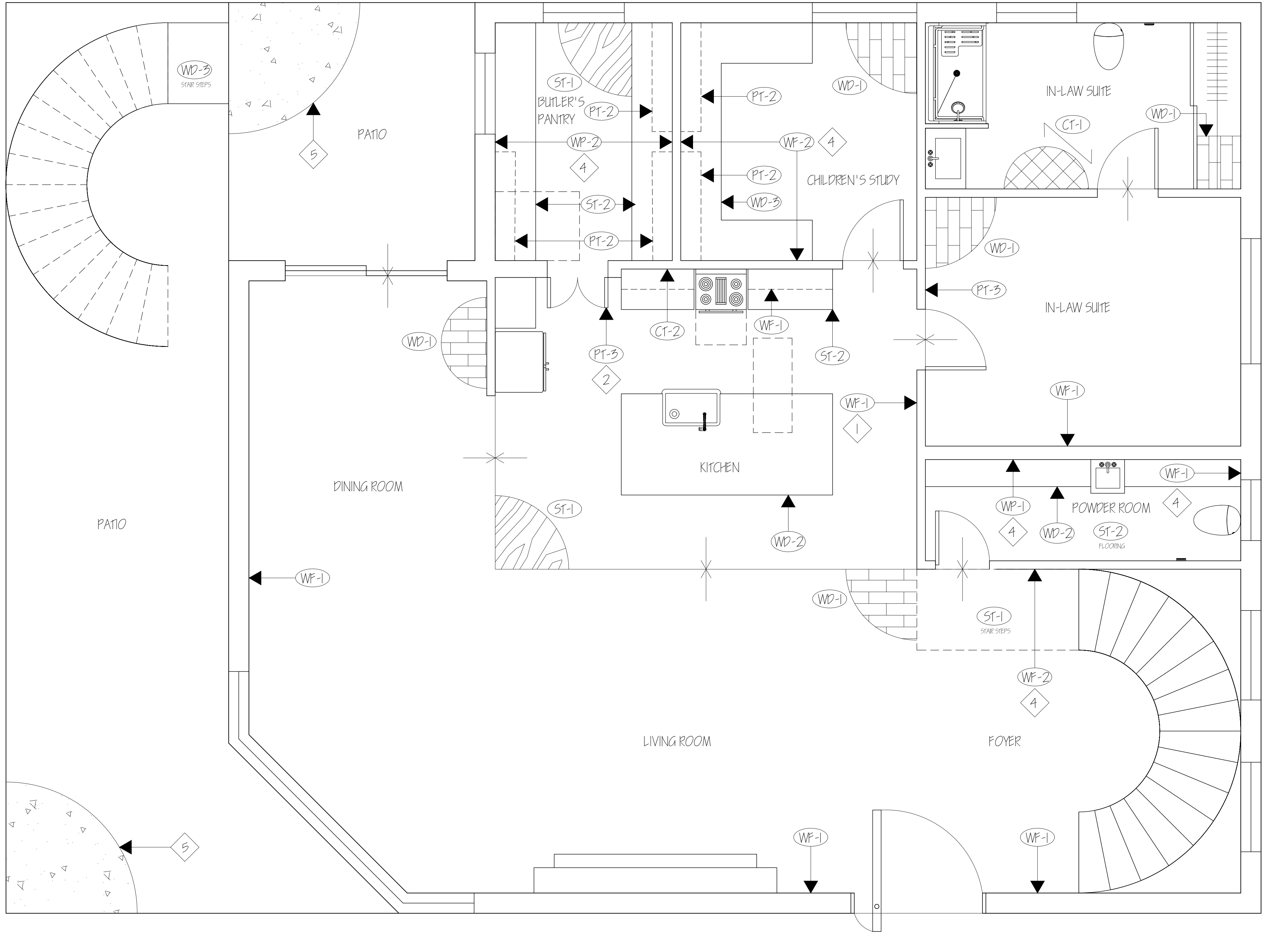
1 1ST FLOOR MATERIAL FINISH PLAN SCALE: 1/4" = 1'-0"
