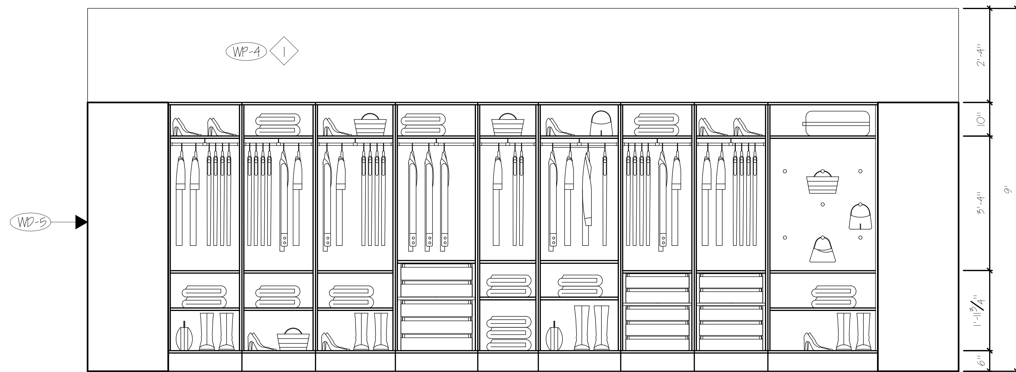
1 MASTER CLOSET FRONT VIEW ELEVATION SCALE: 1/2" = 1'-0"
