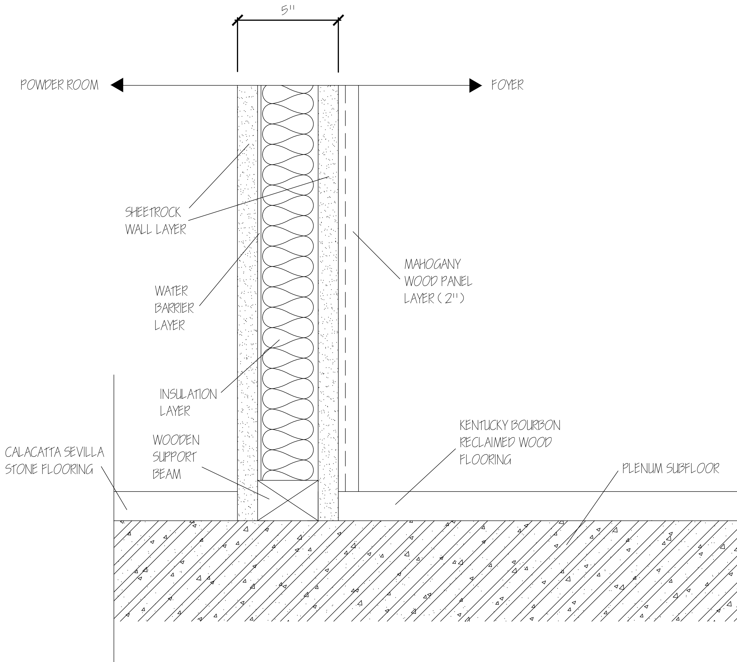
2 POWDER ROOM HIDDEN DOOR PANEL WALL SECTION SCALE: \frac{1}{2} " = 1'-0"
