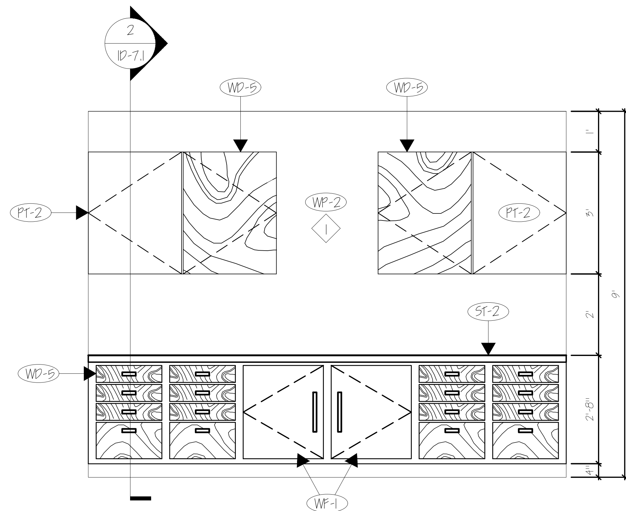
2 PANTRY RIGHT VIEW ELEVATION SCALE: 1/2" = 1'-0"
