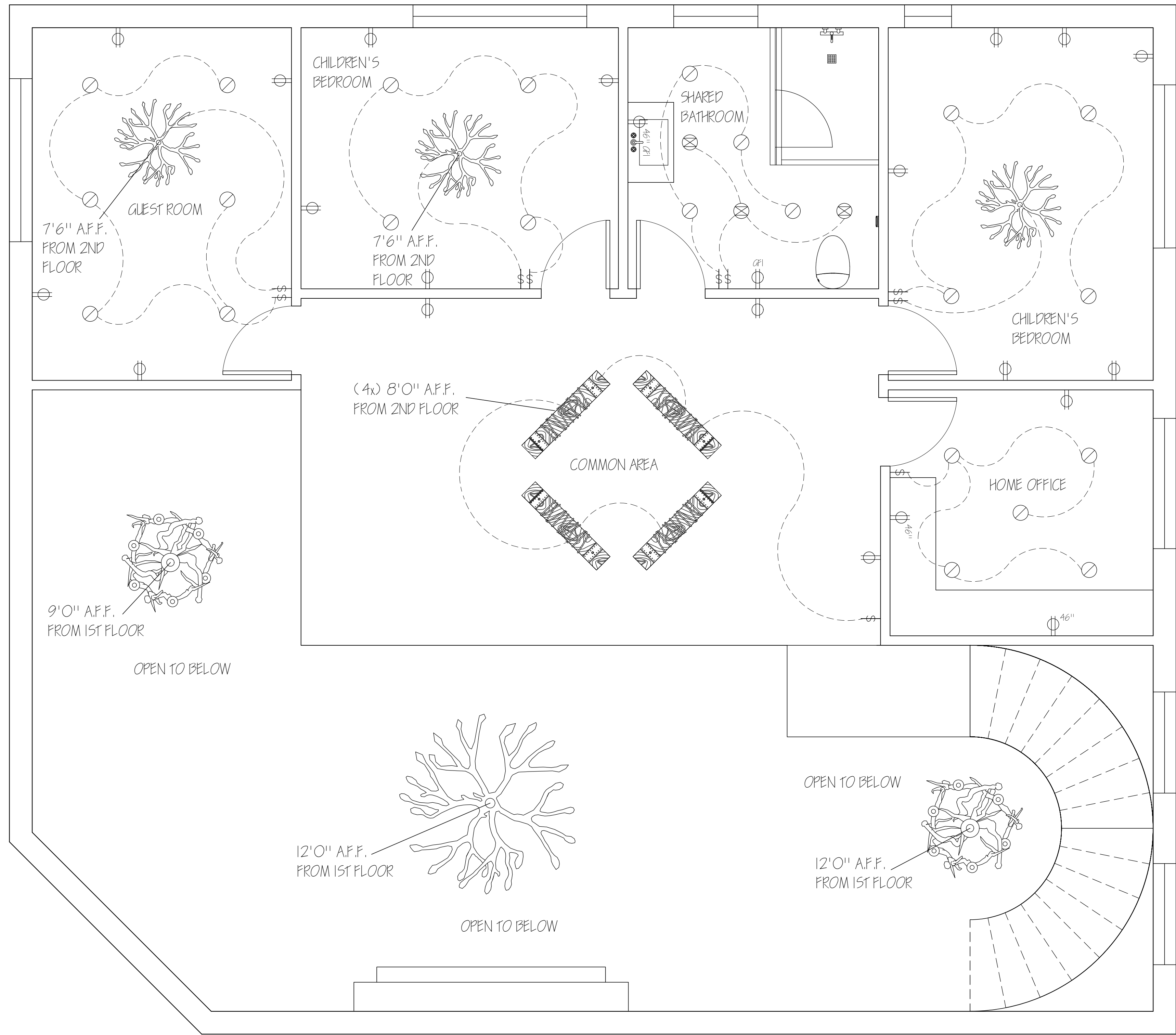
1 2ND FLOOR ELECTRICAL PLAN SCALE: \frac{1}{4}" = 1'-0"
